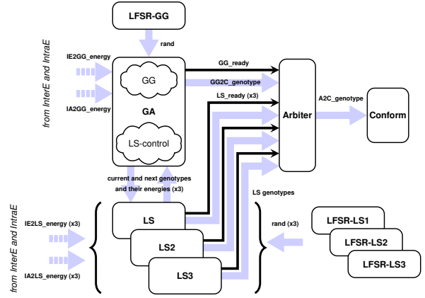
Figure 5 Third development phase: local-search kernels are replicated three times, while an arbiter is added to handle simultaneous energy-calculation requests.
