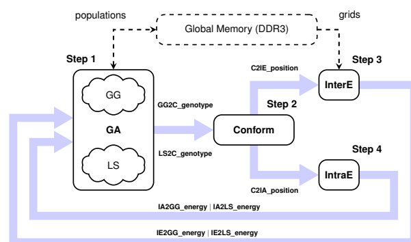
Figure 3 First development phase: initial OpenCL design.
