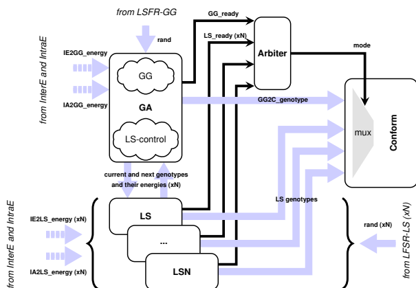
Figure 6 Fourth development phase: local-search kernels are further replicated, while the arbitration mechanism is improved.
