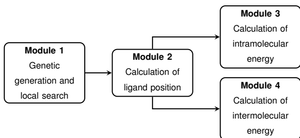
Figure 1 Pipeline processing of the LGA in [11].
