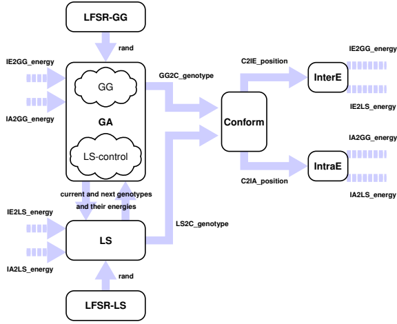
Figure 4 Second development phase: local-search logic is implemented as a separate kernel. From now on, feedback channels are shown as dashed connections, while global-memory accesses are omitted for simplicity.
