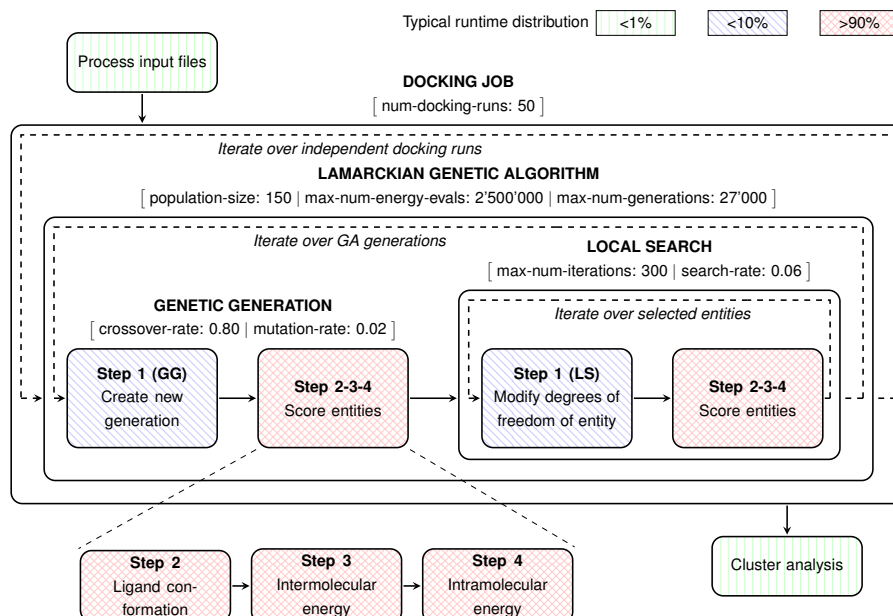
Figure 2 AutoDock Block Diagram [15] with default values of LGA parameters.
