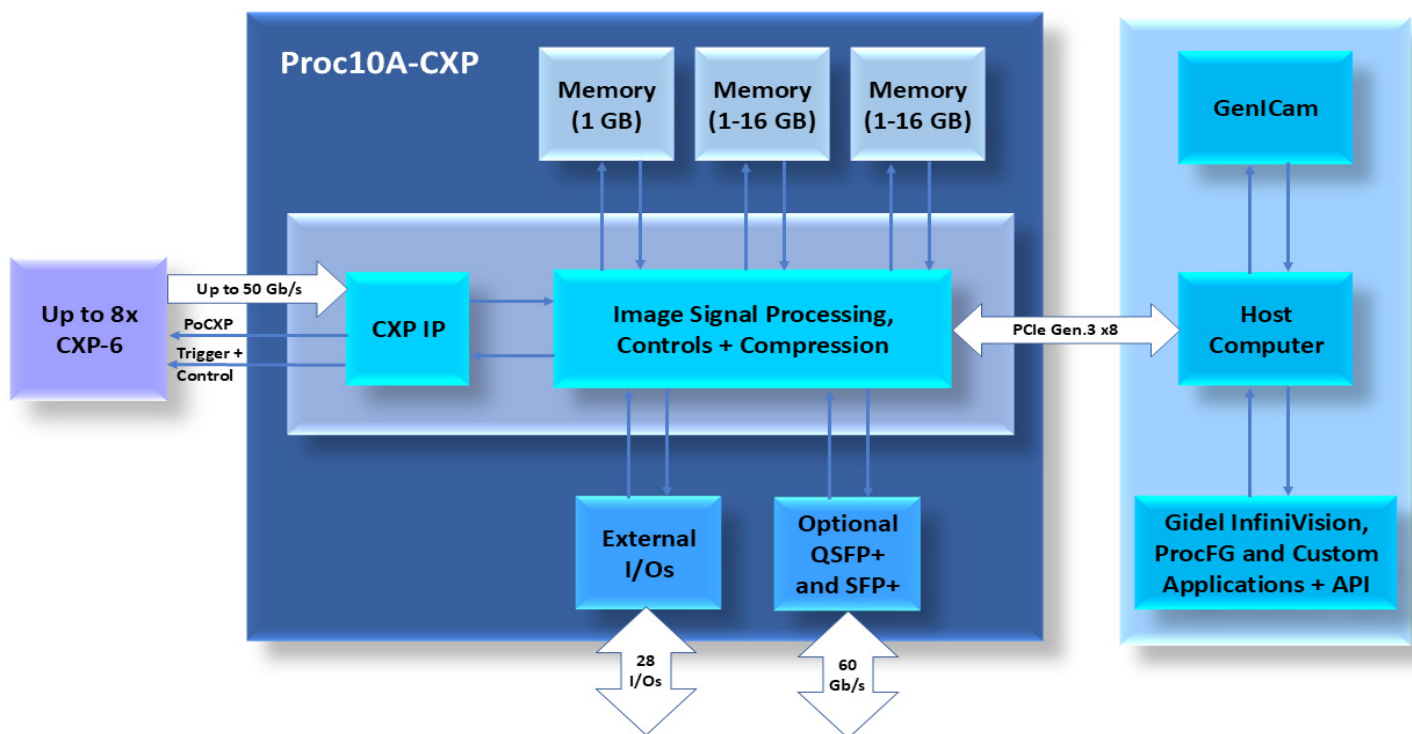
Proc10A-CXP System Block Diagram
